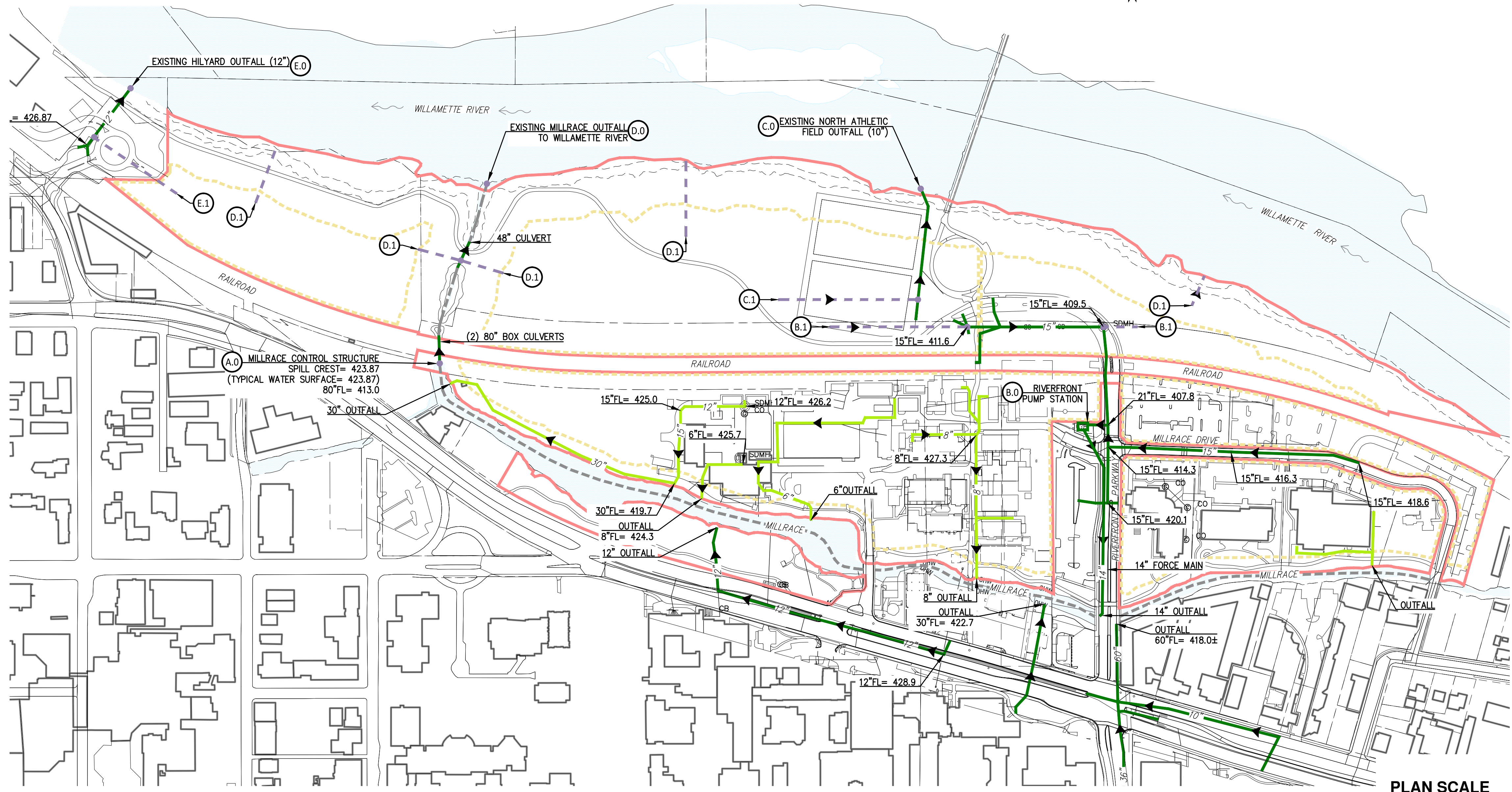
1 STORM DRAIN PLAN
