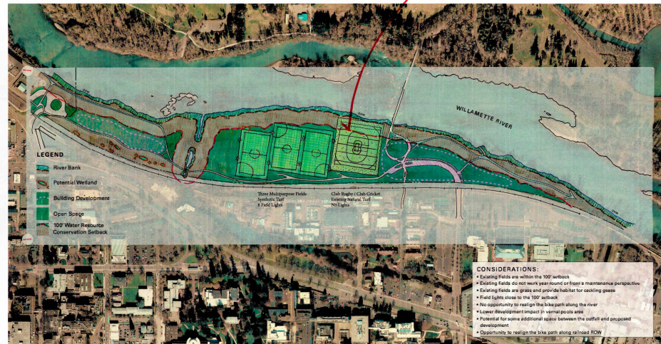
NORTH CAMPUS AREA NORTH CAMPUS CONDITIONAL USE PERMIT PROJECT CONCEPTUAL SITE PLAN OPTION #1 EXISTING FIELDS + THREE NEW FIELDS SCALE 1"=100'
