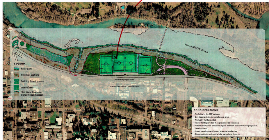
NORTH CAMPUS AREA NORTH CAMPUS CONDITIONAL USE PERMIT PROJECT CONCEPTUAL SITE PLAN OPTION #4 FOUR NEW FIELDS SCALE 1"=100'
